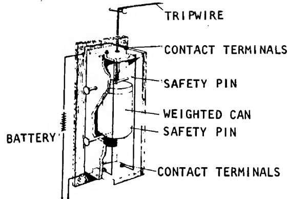
TO ELECTRIC DETONATORS
